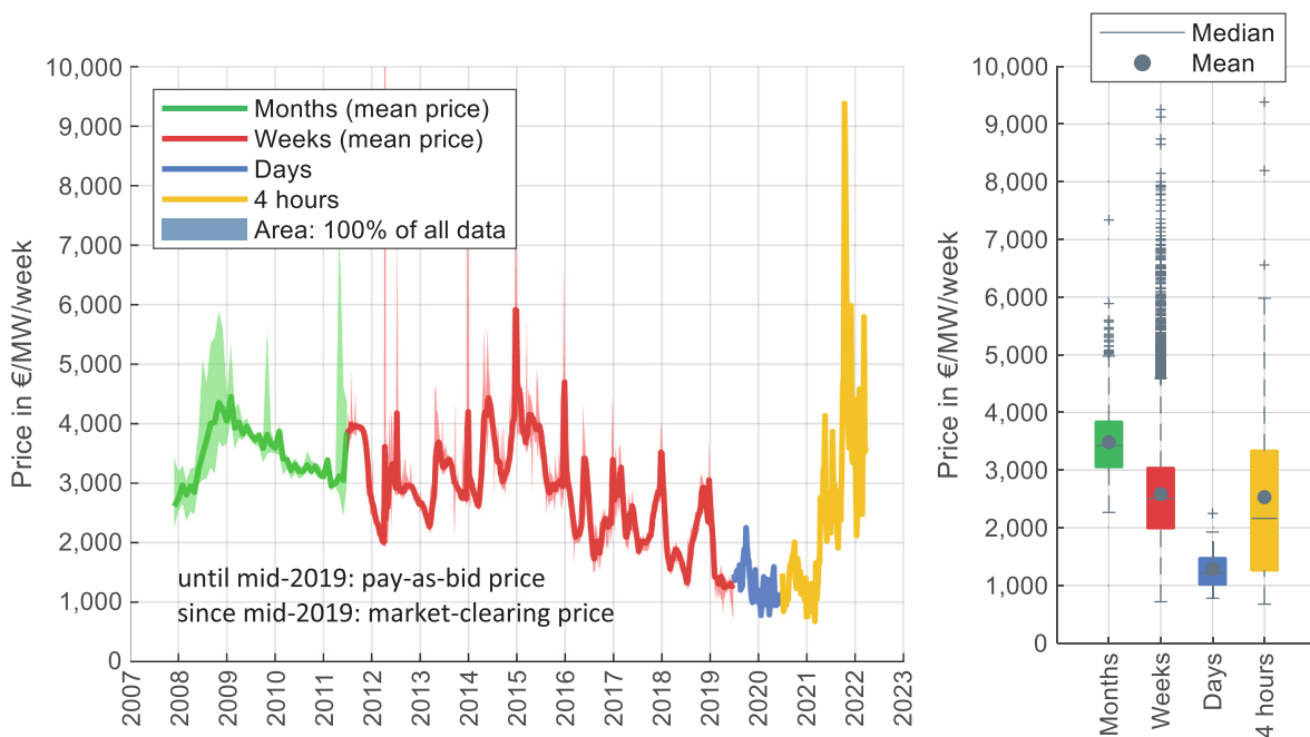
Fig. 14. Left: FCR price development per week until March 2022. Analyzed data from [8]. The prices of the periods of one month, one day and 4 h are scaled to a weekly price for comparability. Therefore, the monthly prices are divided by four, and the daily and four-hourly prices are summed up within the respective week. Right: FCR price ranges for each market design. Analyzed data from [8].
