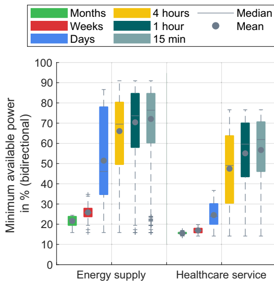
Fig. 18. Available pool power of the EV operating in the chosen sectors over one year.
