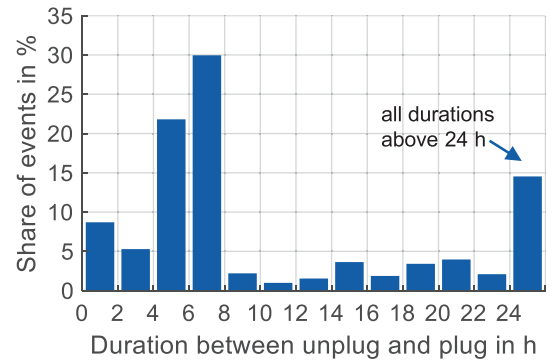
Fig. 4. Duration between unplug and plug (908 measured trips of EVs in healthcare service from database “Measurements”).
