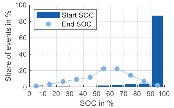
Fig. 5. SOC at unplug and plug (908 measured trips of EVs in healthcare service from database “Measurements”).
